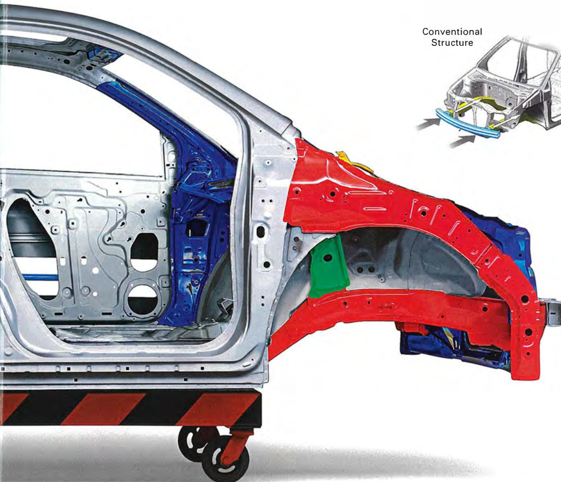
ACE Structure
